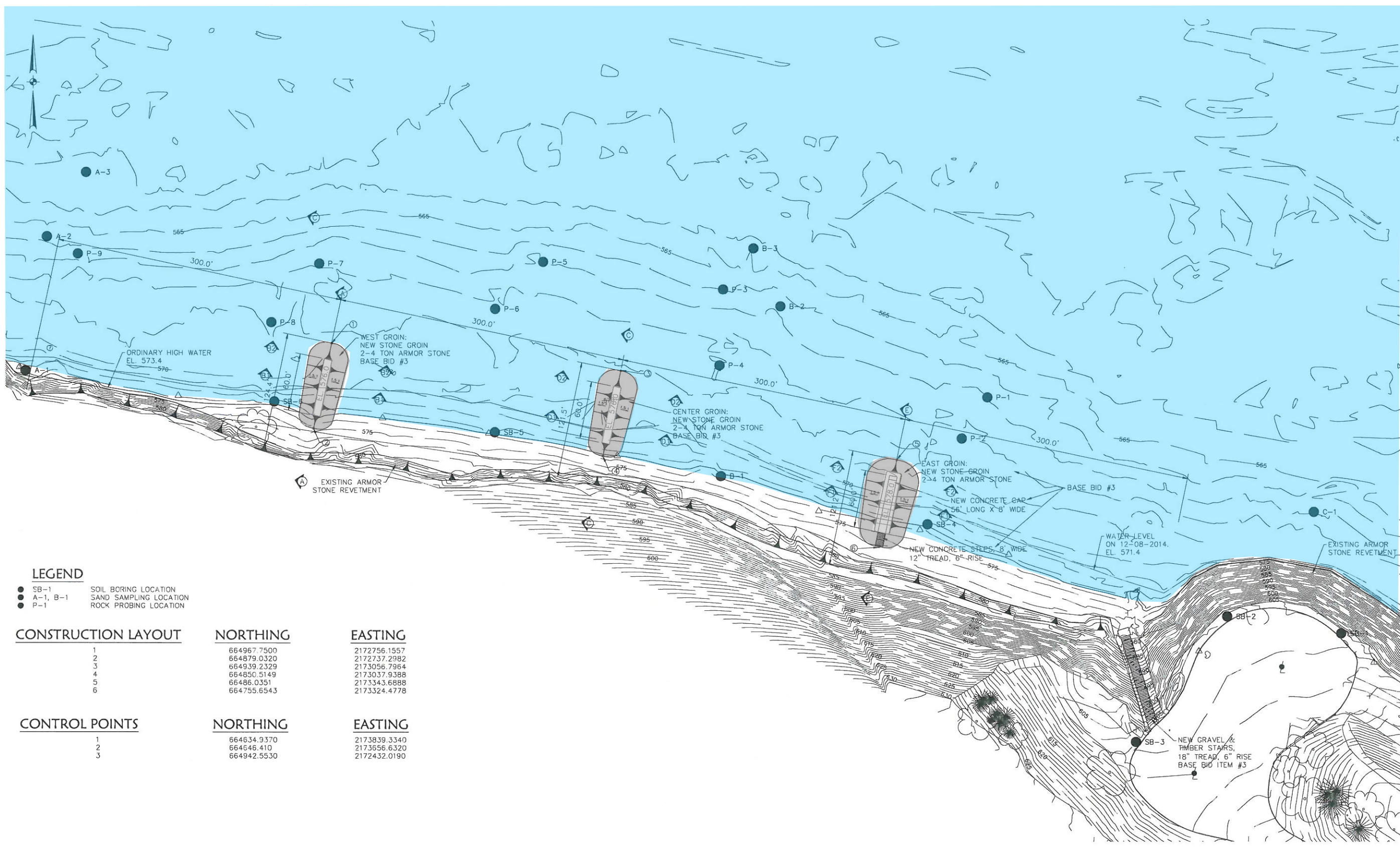
BASE BID 3 SITE PLAN, PERKINS BEACH
